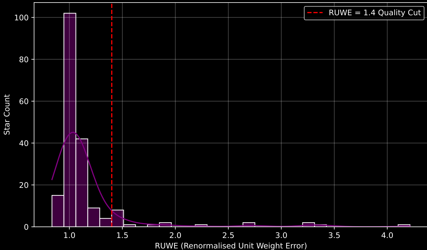
GAPOGEE DR17 Field [K2_C13_181-21_btx] RUWE Distribution (n= 191)
