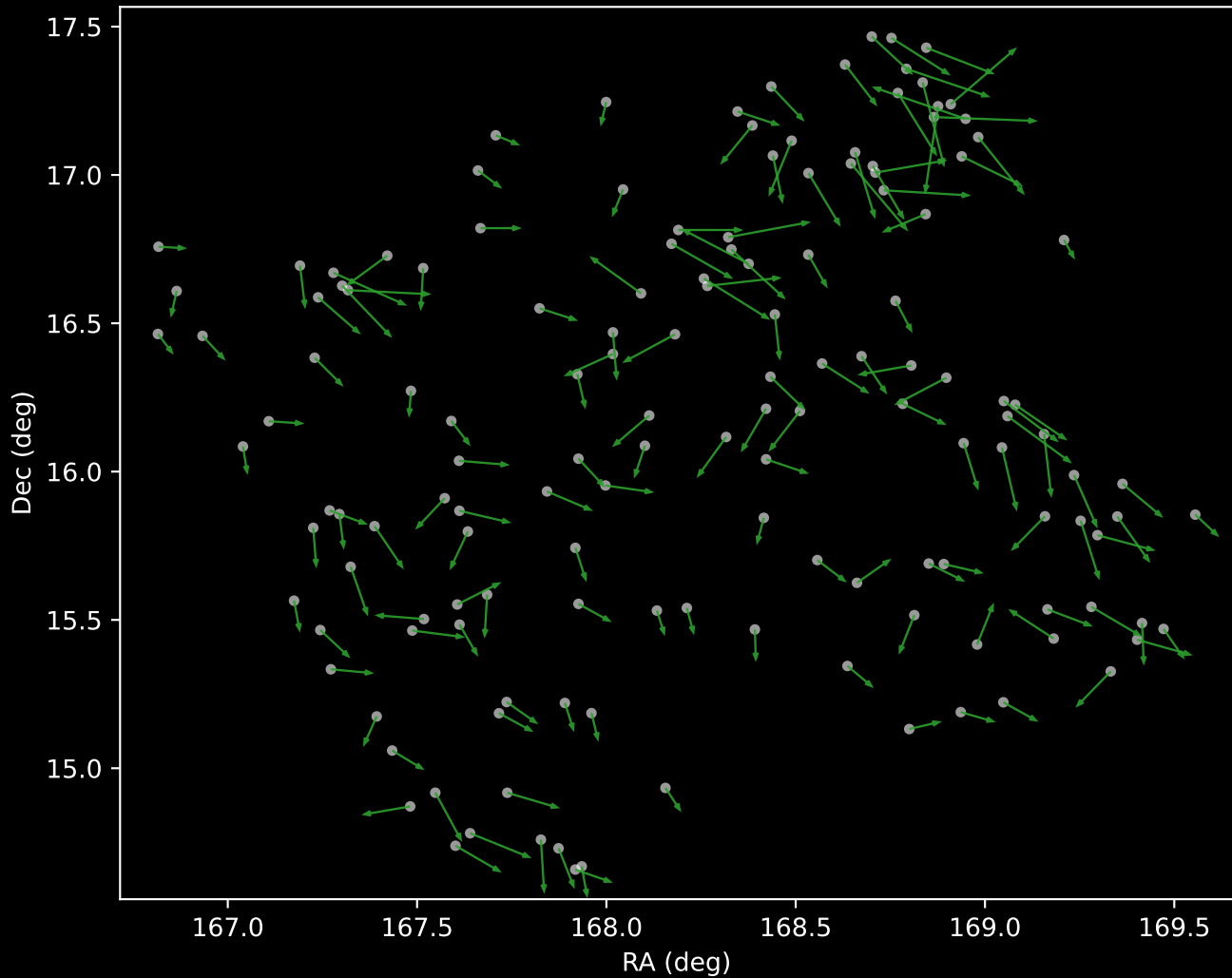
APOGEE DR17 Cluster 4 Proper Motion Vectors (n=147)
