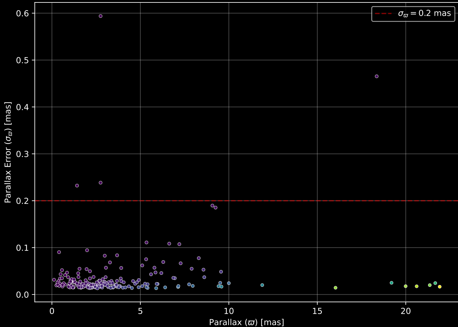
APOGEE DR17 Field: [K2_C13_181-21_btx] Parallax Quality (n= 200)
