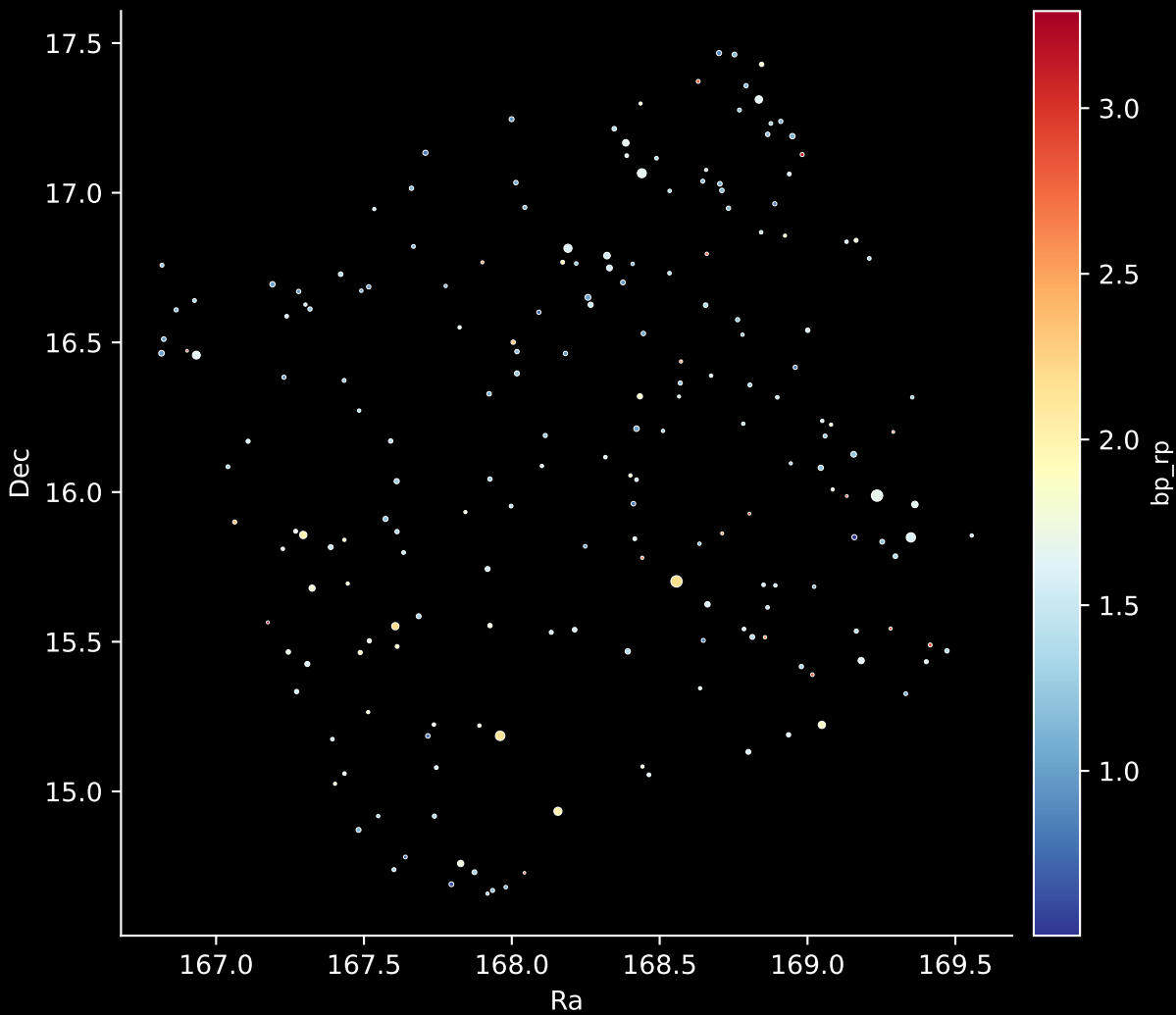
APOGEE DR17 Field: [K2_C13_181-21_btx] Stars: 200
