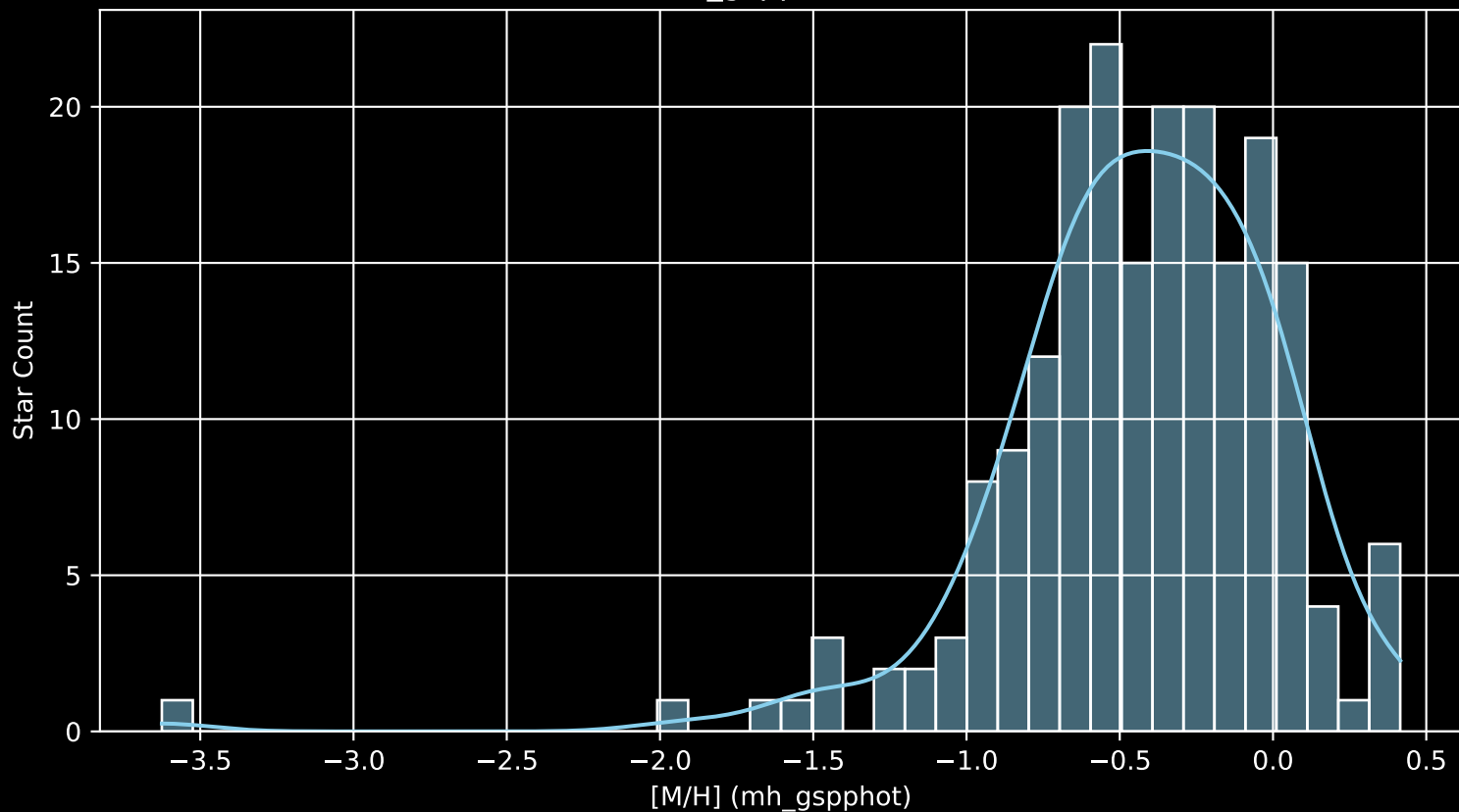
APOGEE DR17 Field: [K2_C13_181-21_btx [M/H] (mh_gspphot) (n= 200)
