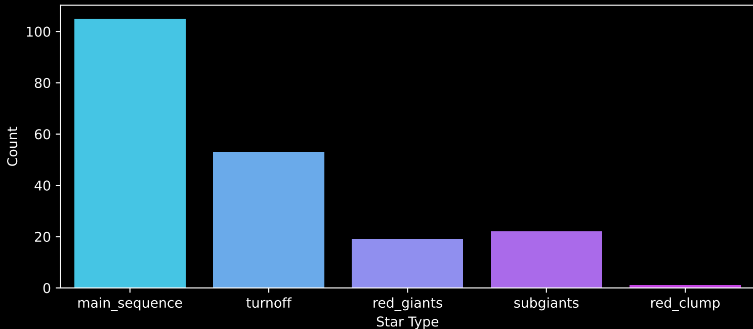
APOGEE DR17 Field: [K2_C13_181-21_btx] Count plot of Star Type
