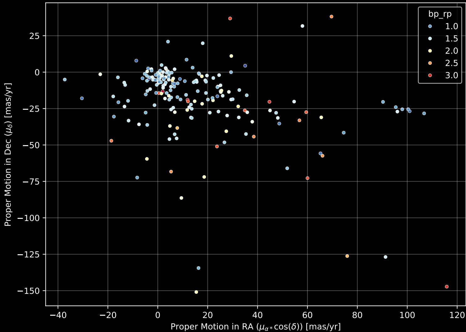
APOGEE DR17 Field: [K2_C13_181-21_btx] Proper Motion Diagram (n= 200)
